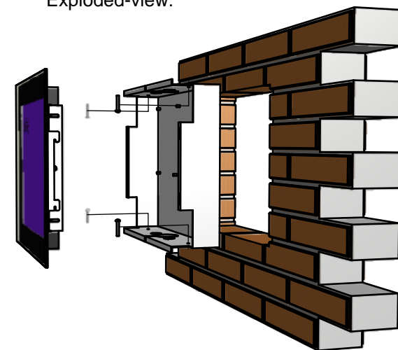
Exploded-view:
