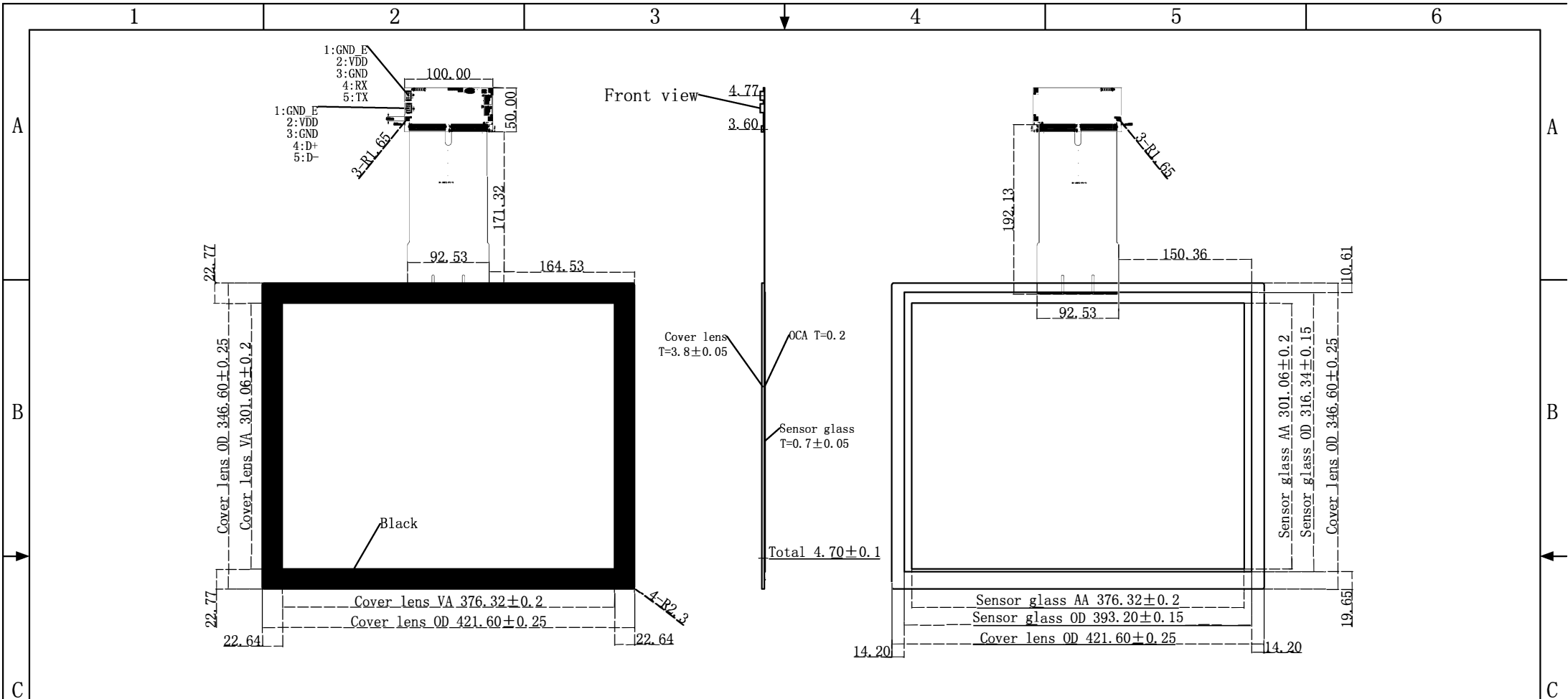
Front View
